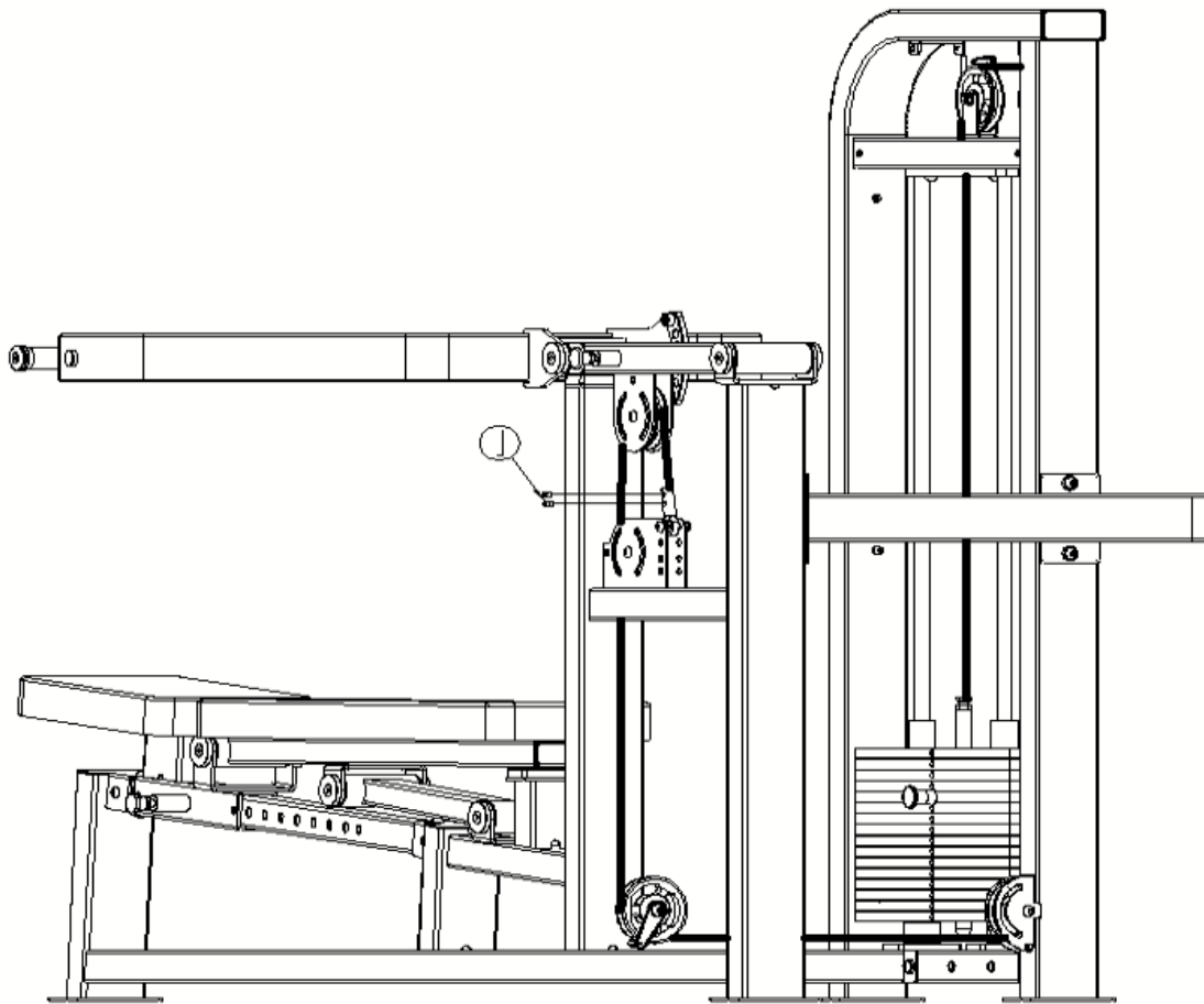
Wire rope alignment diagram
