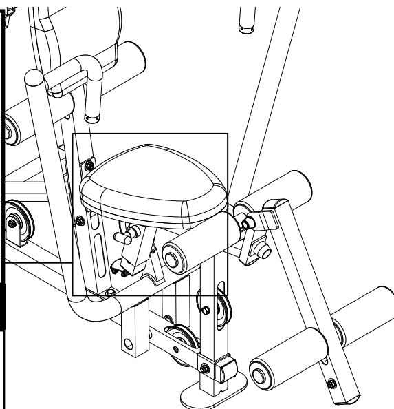
Diagram 1 Seat Pad Adjustment
