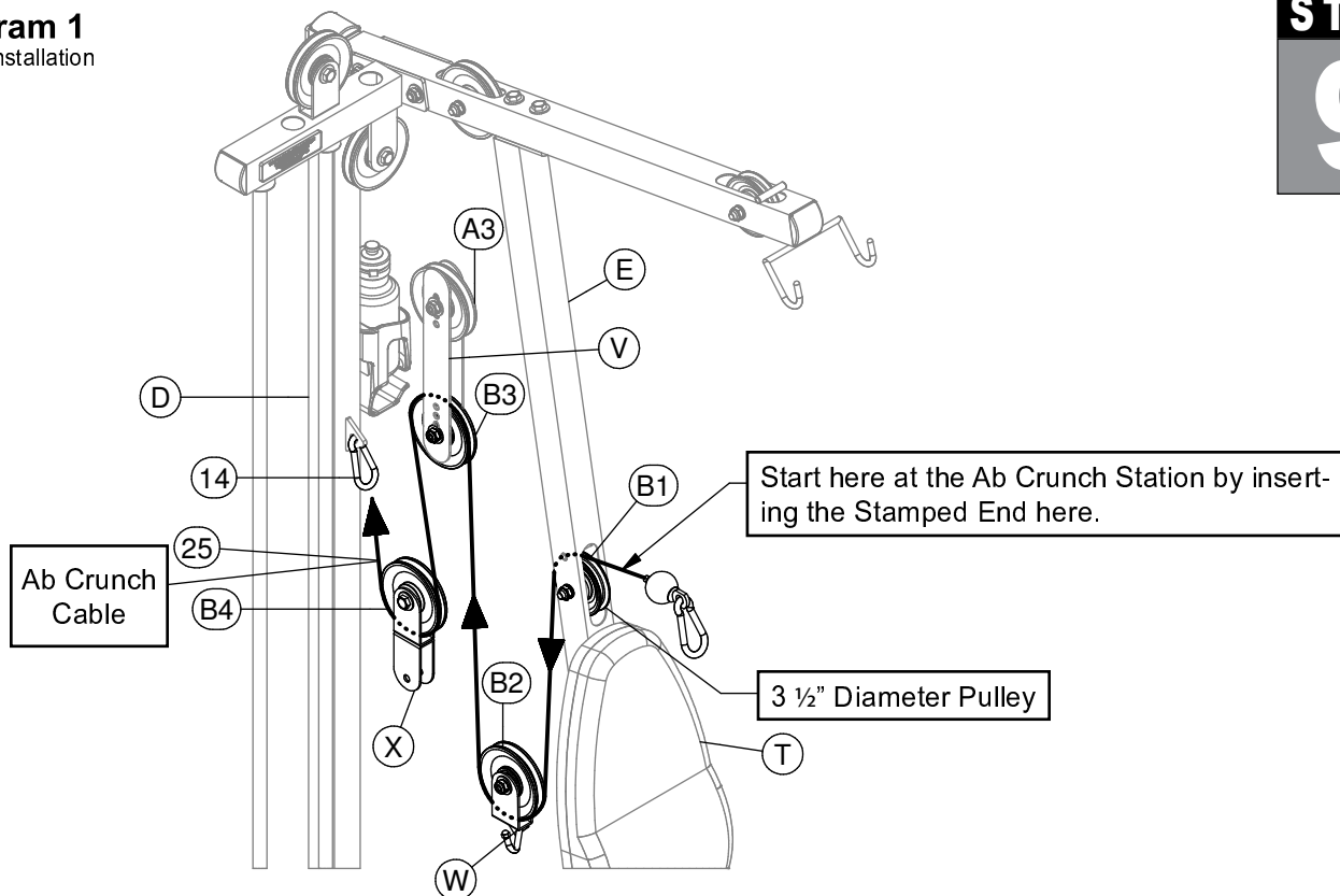
Diagram 2 Pulley Installation
