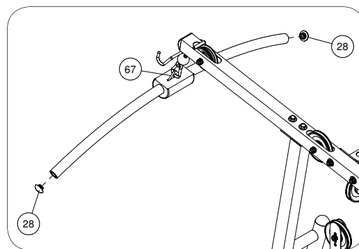
Diagram 4 Lat Bar Installation
