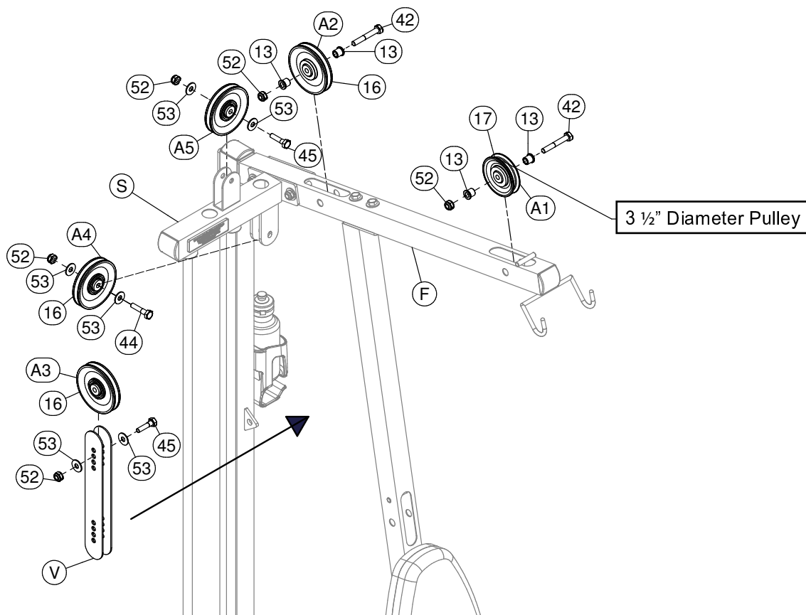
Diagram 2 Pulley Installation
