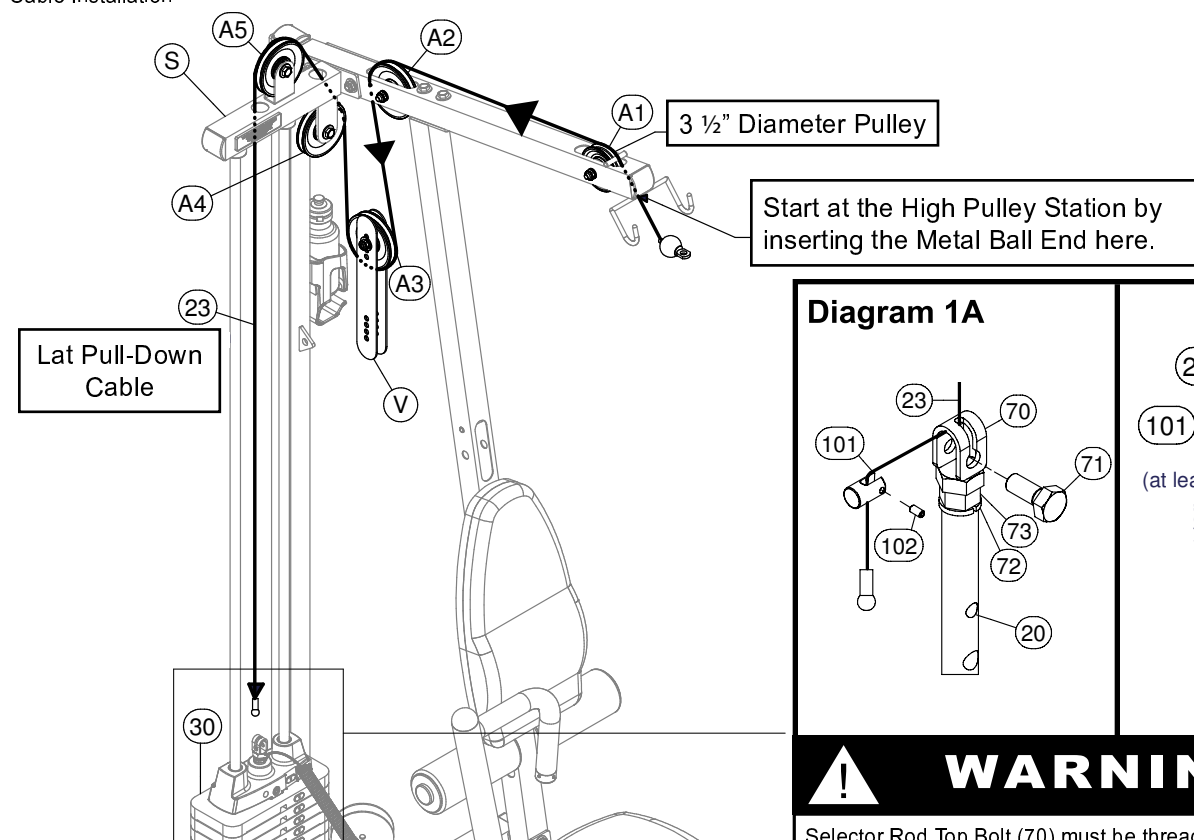
Diagram 1 Cable Installation
