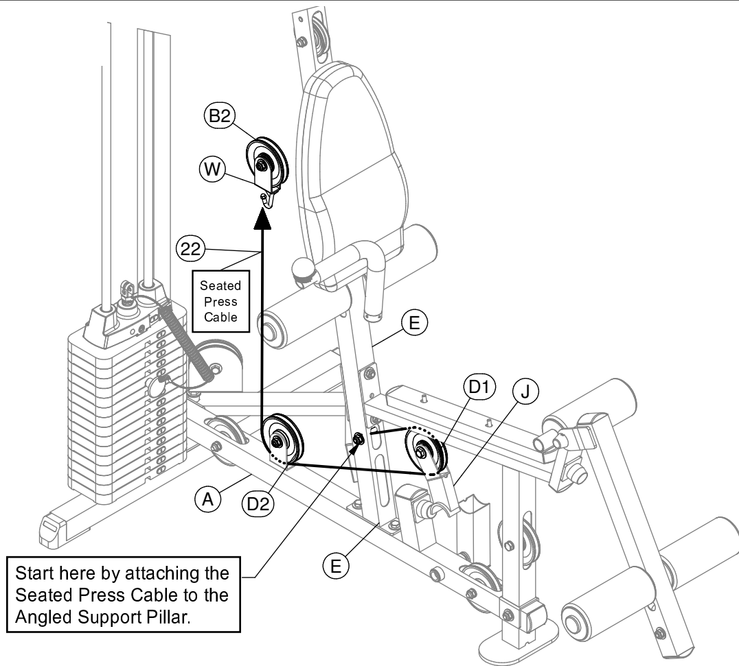
Diagram 1 Cable Installation
