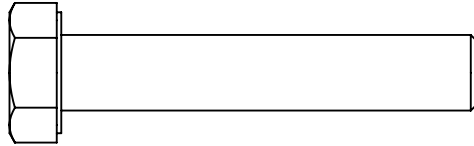
Part #55 HEX HEAD BOLT M10x65mm
